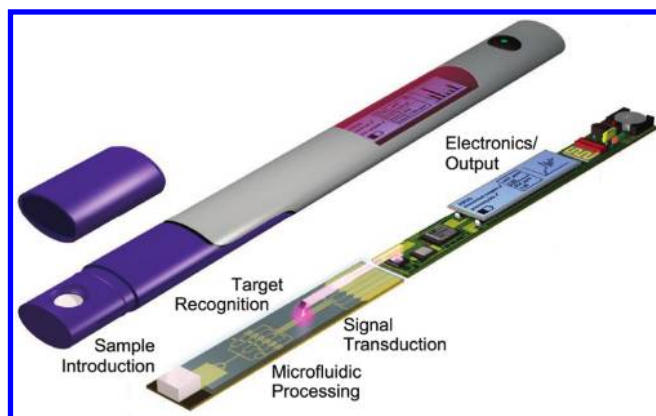
Figure 1. Idealized POC device. Adapted with permission from ref 6a. Copyright 2011 John Wiley & Sons, Inc.
